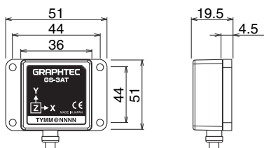
Sensor unit mounting dimensions (Unit: approx. mm)
