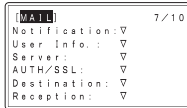
[MAIL Setting]
